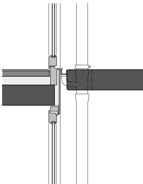
56 Detail Loggia M 1:20
