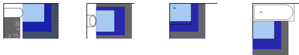
Abb. 16 Movement areas in front of sanitary fittings according to DIN 18022:1989-11, DIN 18025:1992-12 and DIN 18040:2011-09
