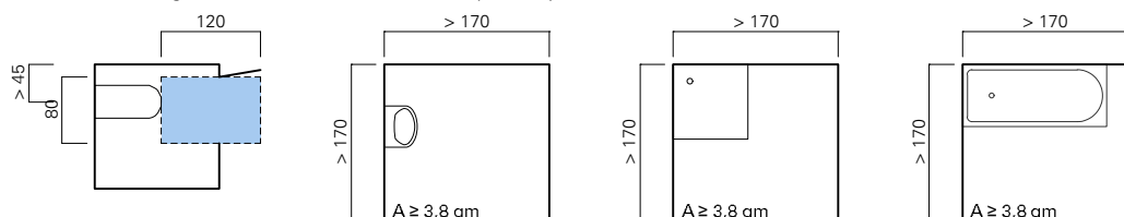
Abb. 15 Adaptable bathroom/shower according to SIA 500:2009, 10.2.1 Swiss requirements to be met by usable and movement areas for an obstacle-free WC or bathroom
